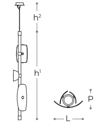
AXI .T1805/SV . design by Patrick Jouin ID Lampada a sospensione - Suspension lamp . p. 38
